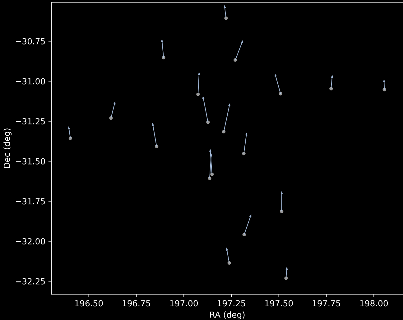
GALAH DR4 Cluster 21 Proper Motion Vectors (n=19)
