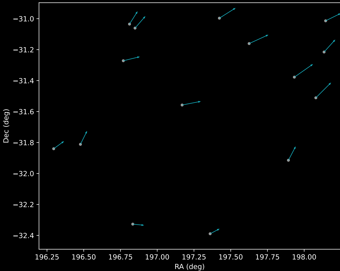
GALAH DR4 Cluster 18 Proper Motion Vectors (n=15)
