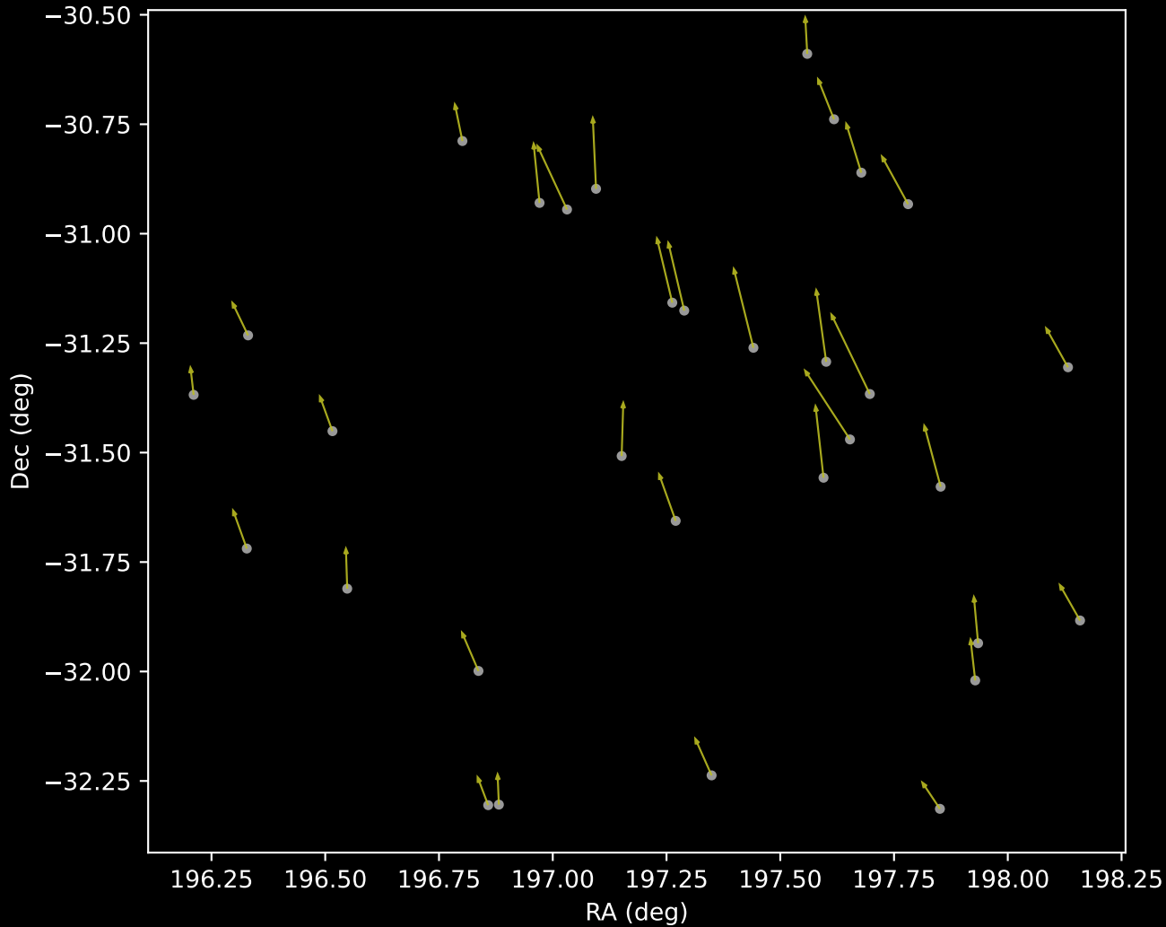
GALAH DR4 Cluster 16 Proper Motion Vectors (n=32)
