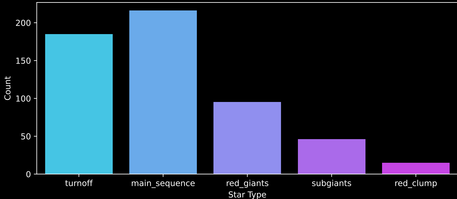
GALAH DR4 Field: [2437] Count plot of Star Type
