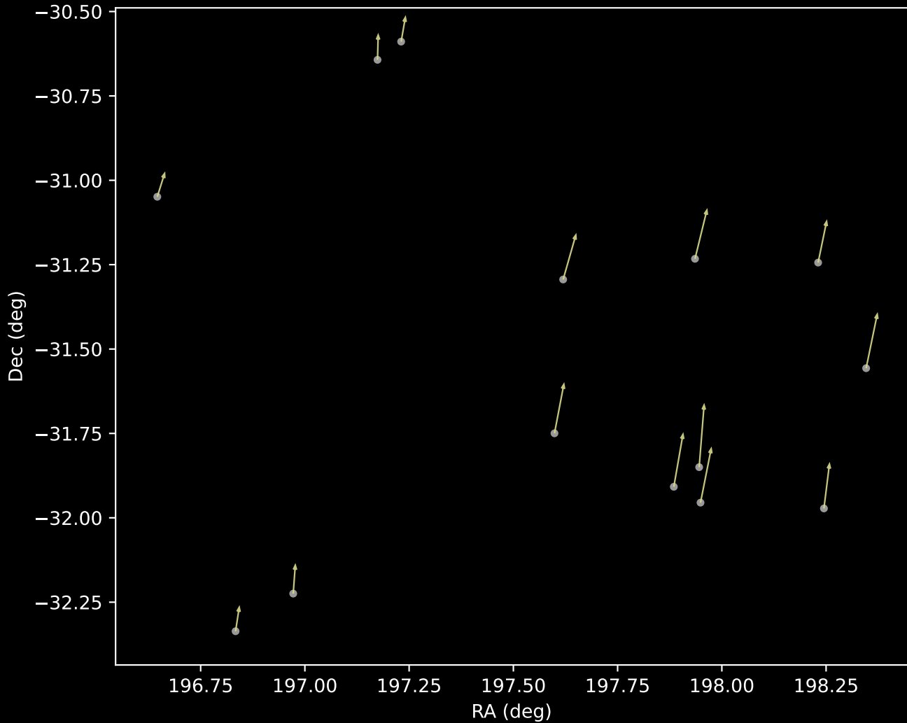
GALAH DR4 Cluster 17 Proper Motion Vectors (n=14)
