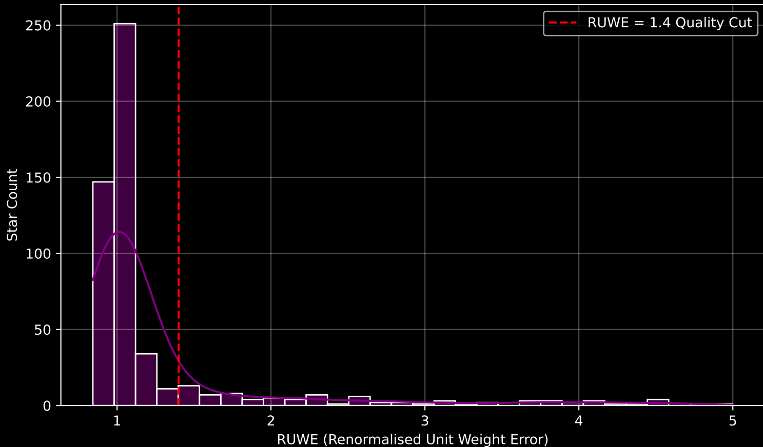
GALAH DR4 Field [2437] RUWE Distribution (n= 528)
